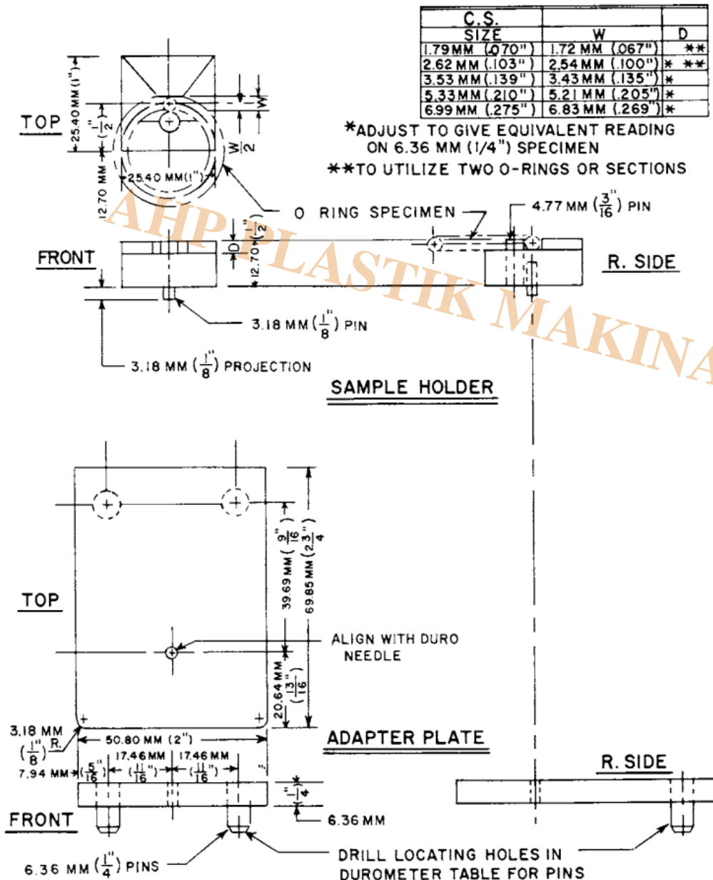
FIG. 2 Holding Fixture for Durometer in Hardness Test
