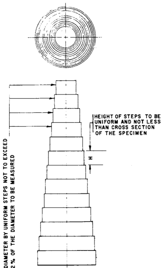
FIG. 1 Stepped Cone Gage
