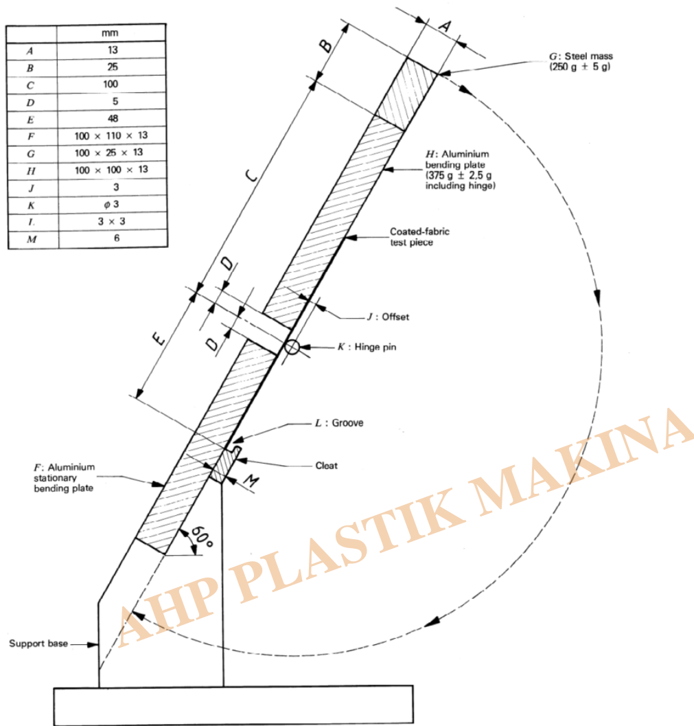
Figure 2 — Dimensions of bending jig
